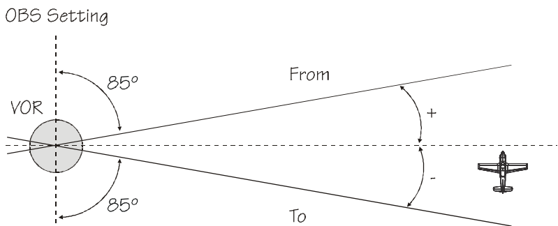
Figure 8 - Cone of Ambiguity
